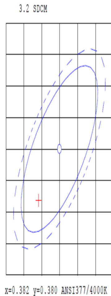
CIE1931 Chromaticity Diagram
